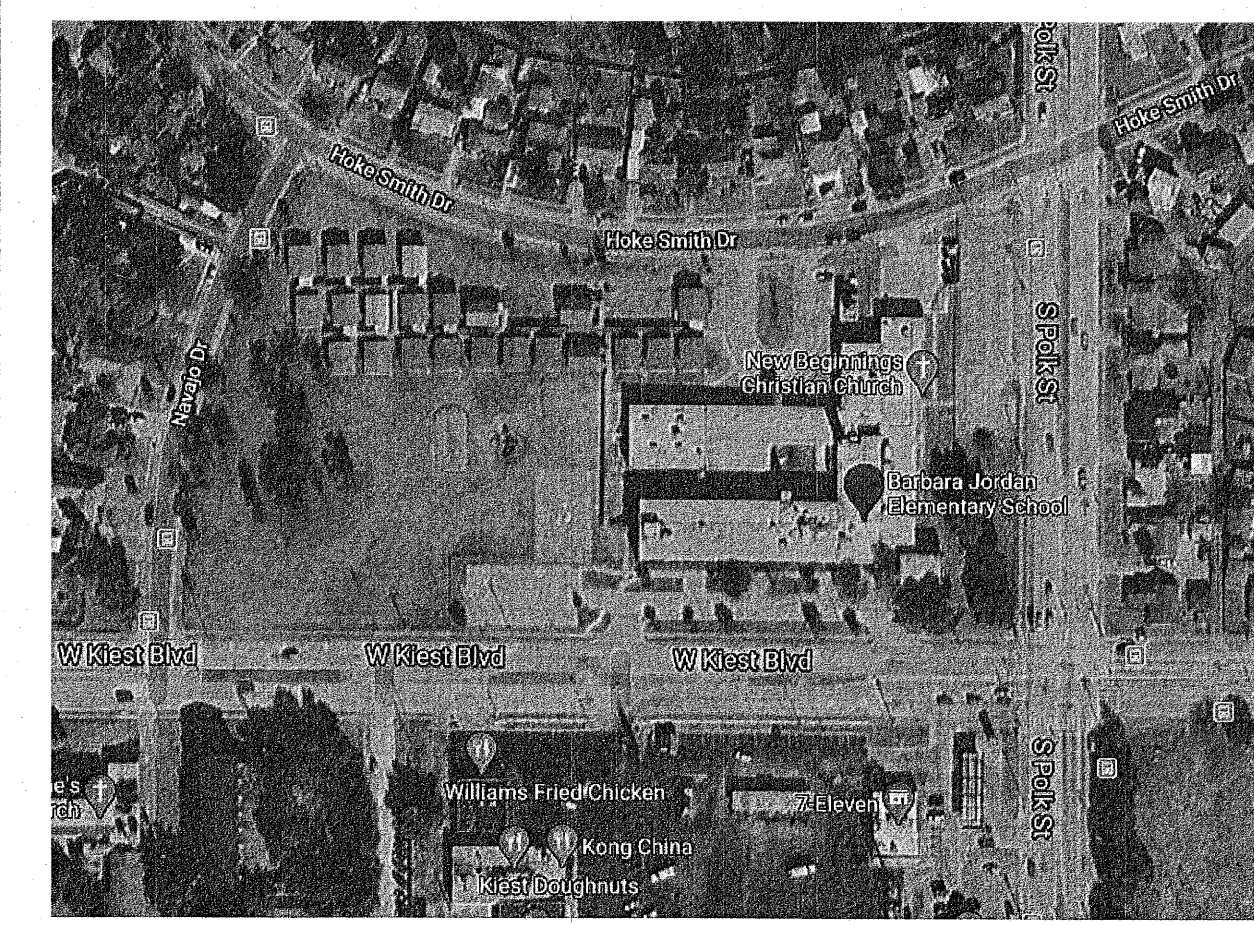
VICINITY MAP
